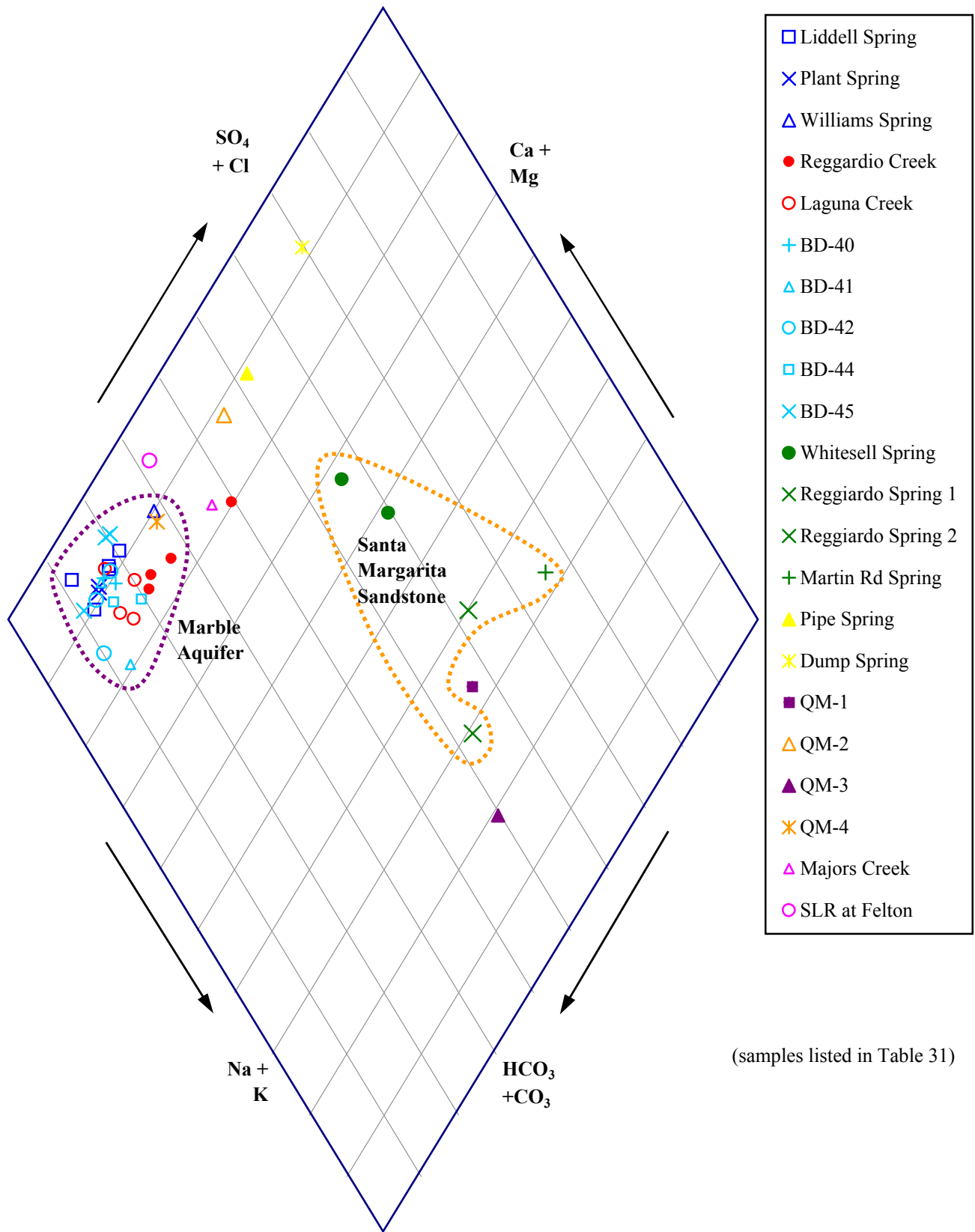
Trilinear Diagram of Bonny Doon Area Ionic Water Types (% meq/L)
